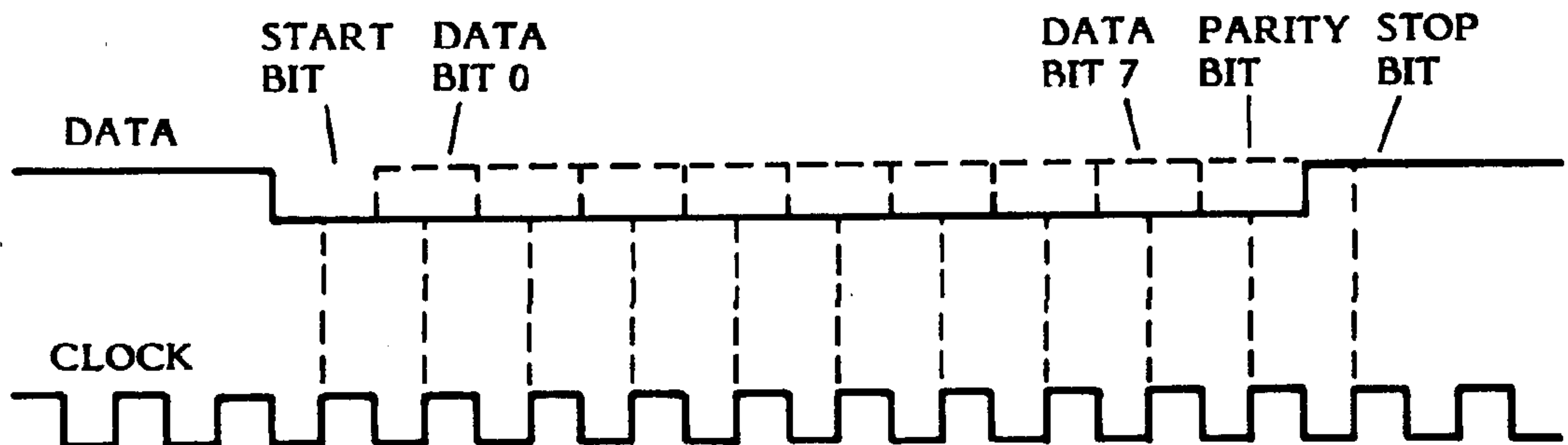
Figure 9-0 DATA FORMAT
