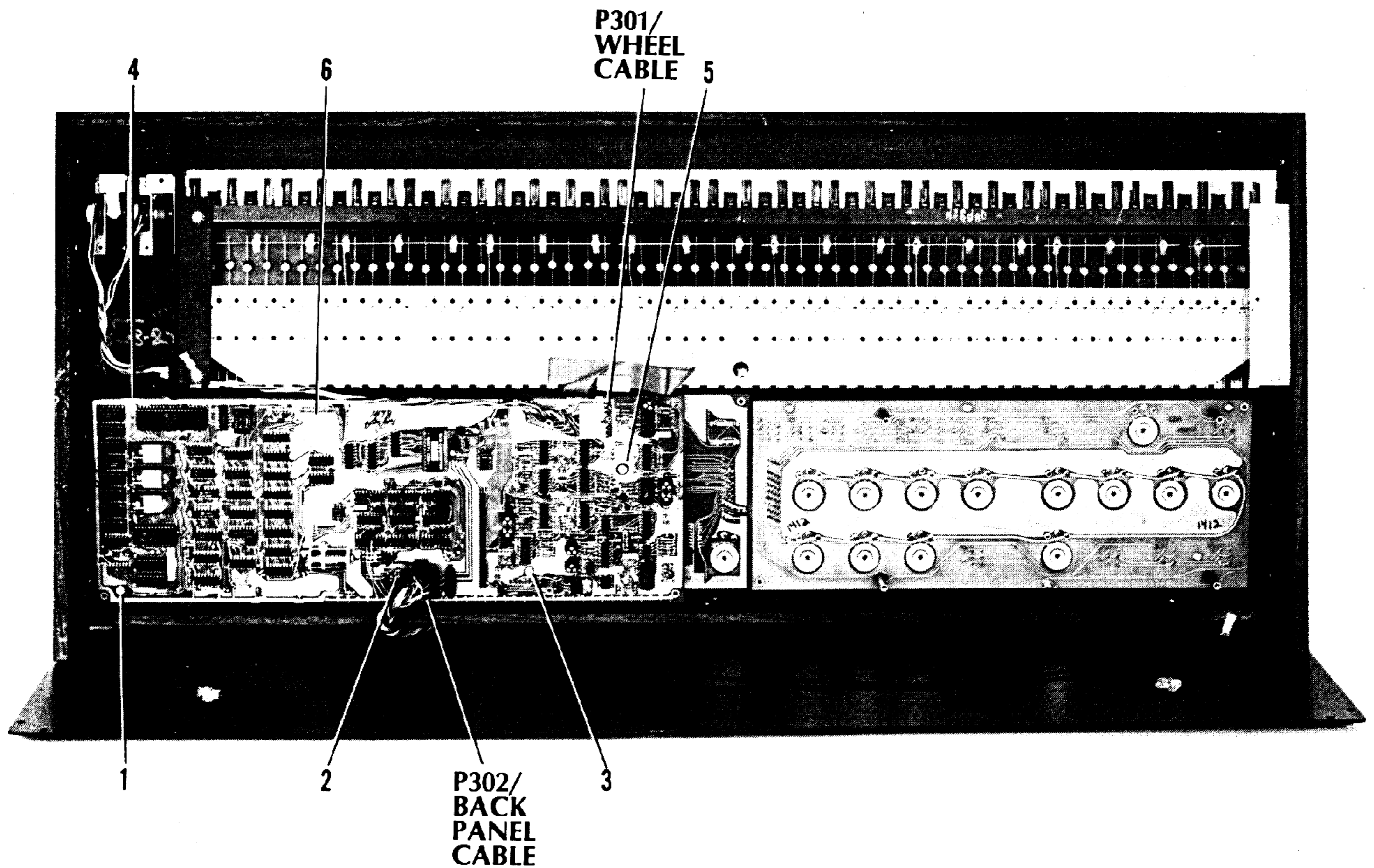
Figure 1-2 PCB 3 MOUNTING
